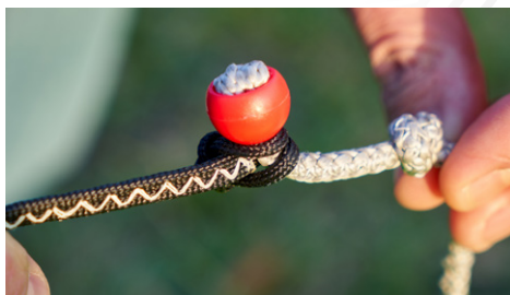
4 - Connect the Front Lines to the Front Grey Line of the Kite. There is no Left/Right sense for the front lines.
